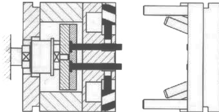
Mold open
