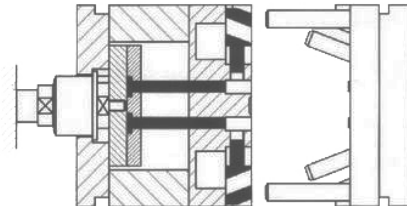
Mold open at the end of process
