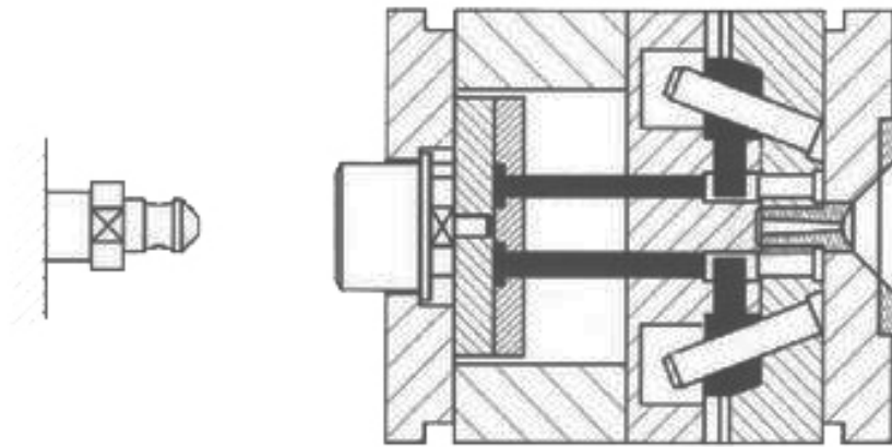
Mold closed
